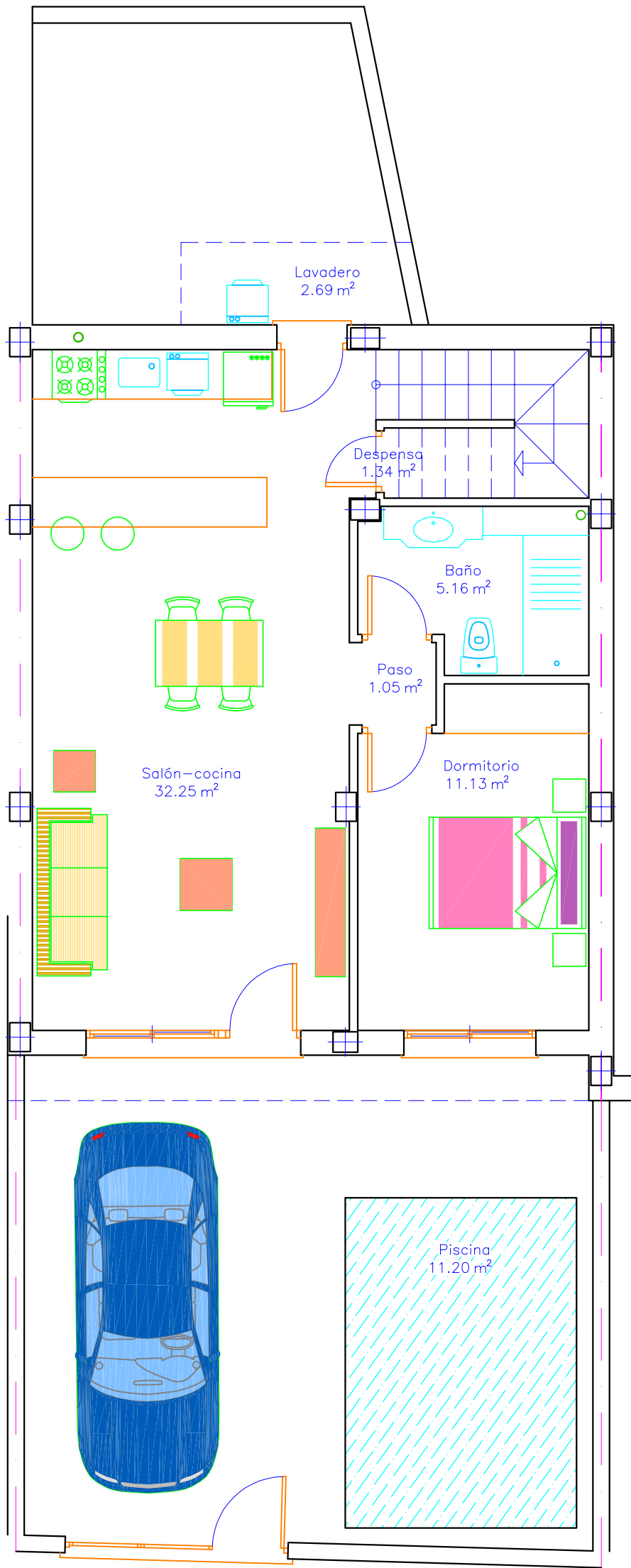
PLANTA BAJA S.C.= 62.30+2.89m 2
